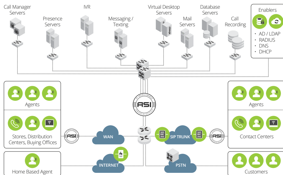
Figure 1: The nGeniusONE platform delivers high level visibility for managing voice, video, and application performance in complex, multivendor retail contact center environments.
